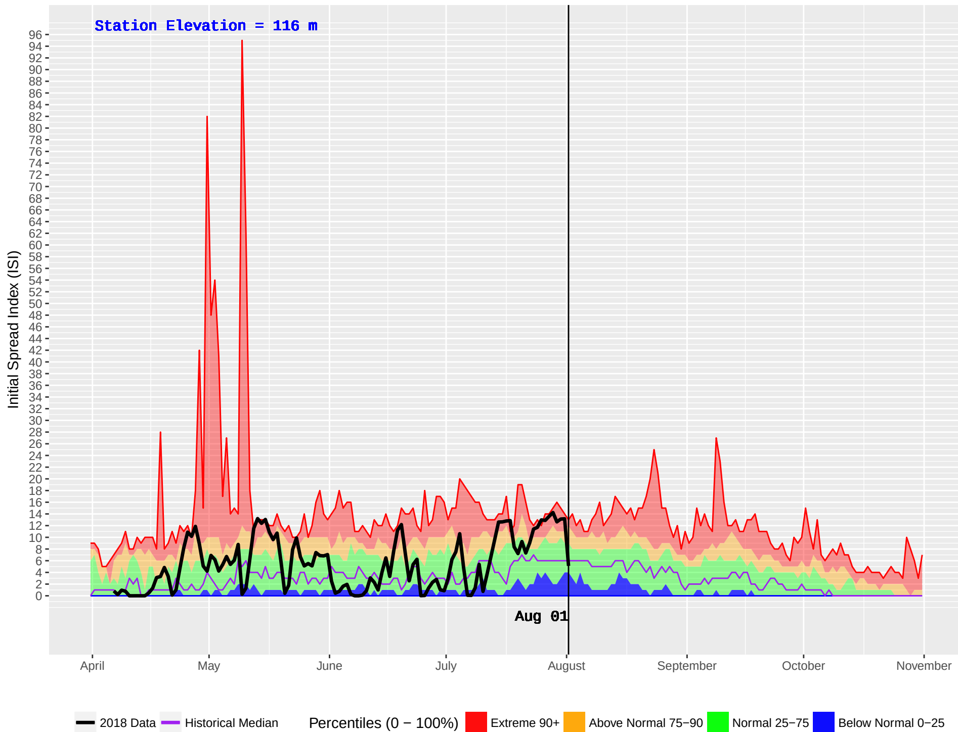
SCAR CREEK (82) : Historical (1982–2016) and Current (2018) Daily Initial Spread Index (ISI)
