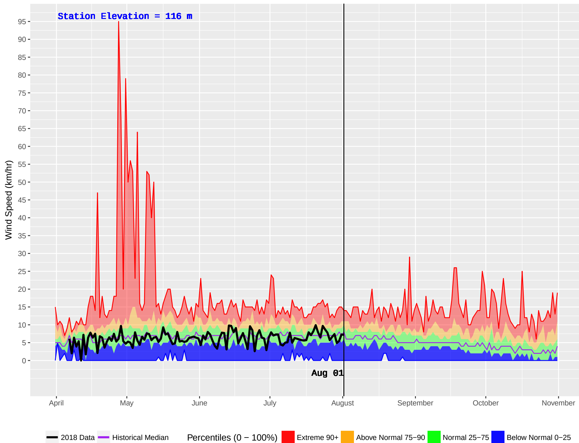
SCAR CREEK (82) : Historical (1982–2016) and Current (2018) Daily Wind Speed
